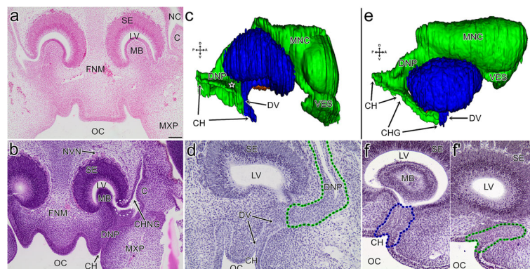
Fig. 2 Transverse sections ( a , b , d , f and f ) through the snout and 3D reconstructions ( c and e ) of the vomeronasal organ and associated structures of the grass snake embryos at different developmental stages. a The vomeronasal organ at the end of developmental stage II. b The vomeronasal organ at the end of developmental stage II. The dashed line indicates the connection of the VNO with the nasal cavity. c The medial aspect of the vomeronasal organ (blue) and its relation to the nasal cavity (green) and the lacrimal duct (orange) at the beginning developmental stage IV. The star indicates the area of the future fusion between the maxillary process and the frontonasal mass. d The connection between the primordium of the vomeronasal organ and the developing nasopharyngeal duct at the beginning of developmental stage IV. e The medial aspect of the vomeronasal organ and its relation to the nasal cavity and the lacrimal duct at developmental stage V. The colours of the structures are the same as in the c. f The embryonic vomeronasal organ and its duct (blue dashed line) at developmental stage V. f The choanal groove (green dashed line) at developmental stage V. Seven sections posterior to f. Abbreviations: C concha of the nasal cavity, CH choana, CHG choanal groove, CHNG Choanengang, DNP nasopharyngeal duct, DV duct of the vomeronasal organ FNM frontonasal mass, LV lumen of the vomeronasal organ, MB mushroom body, MNC main nasal cavity, MXP maxillary process, NC nasal cavity, NVN vomeronasal nerve, OC oral cavity, SE sensory epithelium of the vomeronasal organ, VES vestibulum. Scale bars 100 \mu m ( a , b ); 50 \mu m ( d , f and f ). 3D reconstructions are not scaled
