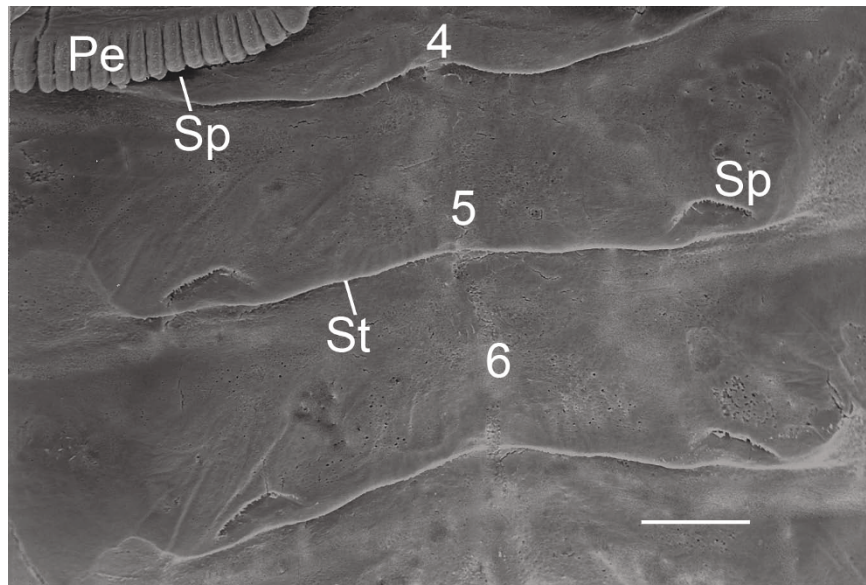
Figure 1 Ventral view of embryo opisthosoma with spiracles (Sp) and small flap-like sternites (St) starting to form. Centruroides gracilis , supine. SEM. The spiracles evident here are near the posterior margin of segments 4, 5 and 6. The spiracles on segment 4 are only partially visible because the pectines (Pe) from segment 3 still overlap on the ventral surface of segment 4. The spiracles are open with no closing mechanism until after the first molt (second instar). Scale, 200 \mu\text{m} .
