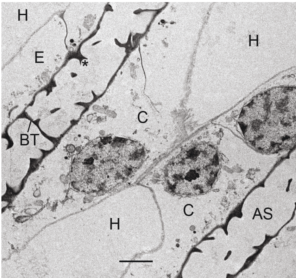
Figure 17 Presumptive primordial space holder across the hemolymph channel (H) of a second instar book lung. Centruroides gracilis . TEM. Many cells deteriorate in the primordial hemolymph channel (Figs. 12, 16), resulting in space for passage of hemolymph. The two intact cells (C) shown here make contact across the channel lumen. These may be precursor pillar cells for the pillar type space holders that earlier workers report are a common feature in the book lung hemolymph channels of adult scorpions and spiders [30,45,47-50]. AS, air sac; BT, bridging trabeculae; asterisk, non-bridging trabecula. Scale, 2 \mu m.
