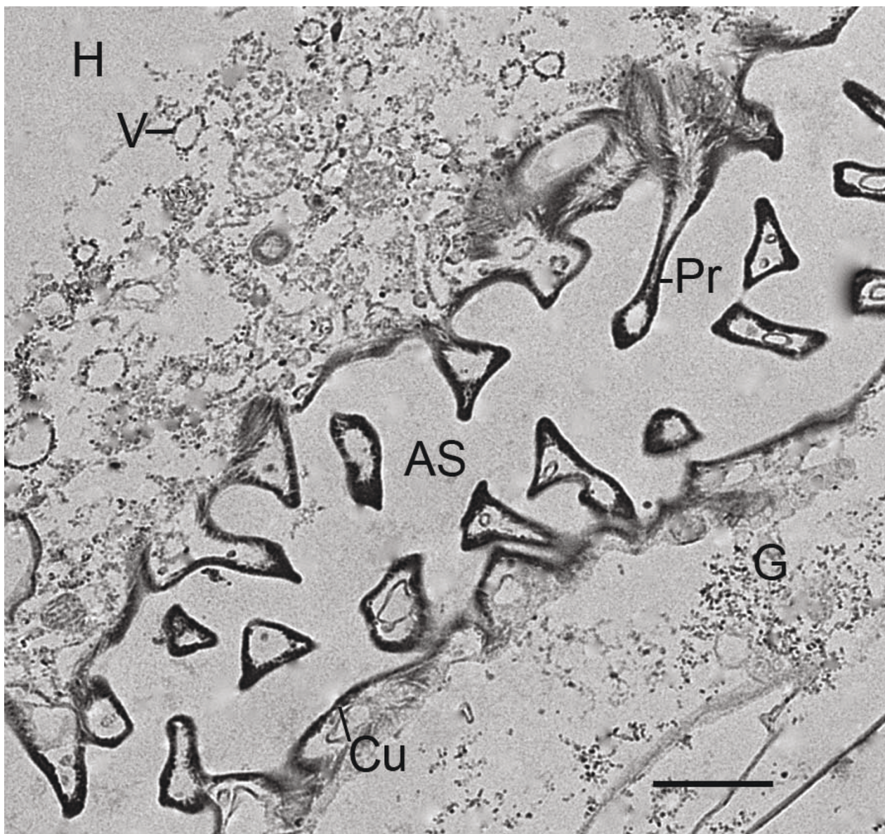
Figure 14 Formation of space holders by extension of cell processes (Pr) into the lumen of the developing air sacs (AS). First instar, Centruroides gracilis . TEM. Cells adjacent to the air sac wall contain many vesicles (V) and granules (G) that are apparently components for the thickening cuticular wall (Cu). The cell processes (trabeculae) also contain vesicles and granules so apparently the protrusions can gradually enlarge and extend across the lumen, forming wall-to-wall (bridging) space holders (e.g., Figs. 15, 16, 17). H, primordial hemolymph channel. Scale, 1 \mu m.
