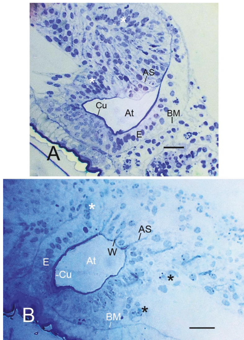
Figure 2 Proliferation and migration of precursor book lung cells from the invaginated epithelium (E) of the atrium (At). Light micrographs (LM), ventral views, semi-thin sections. Centruroides gracilis . A. Newborn first instar. The air sacs (AS) in this book lung are at an early stage and barely discernible. Little or no widening is evident at the atrial origin of the air sacs. The cuticular wall (Cu) of the atrium is absent or very thin at the sites where air sacs are forming. The epithelial cells of the atrial wall are in a distinct layer where lamellae are not being formed; a basement membrane (BM) is present at the basal surface of these cells. The cells in the epithelial layer toward the left in the photo are more numerous as though proliferating near the site where air sacs are forming. On either side of the region of developing air sacs, the basement membrane is absent or disrupted and the precursor cells appear to be migrating inward (asterisks). B. Embryo book lung with some air sacs more advanced than those in Figure 2A. Inside the wall of the atrium, epithelial cells (E) of the hypodermis form a layer with a basement membrane (BM) at their basal surface. The cuticular wall (Cu) of the atrium is much thinner at the site where air sacs are forming. The primordial air sacs (AS) separate aligned precursor cells into double rows. Some cells (asterisks), not yet aligned into rows, appear to be dispersing inward from the atrial epithelium, and at these sites the basement membrane is disrupted or absent. Some widening (W) of the air sac entrance is evident at the atrial origin of two air sacs. In the lateral region (right) of the book lung, the developing air sacs are barely evident among cells not yet aligned. Scales, 20 \mu m.
