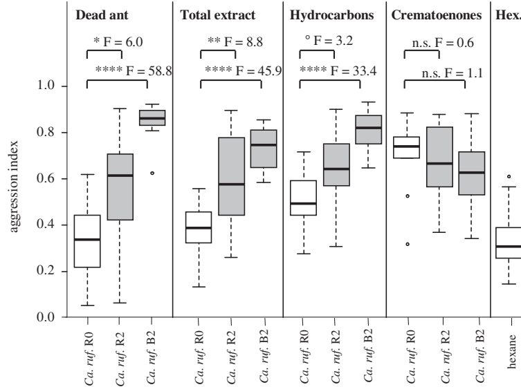
Figure 5 Aggression of Crematogaster modiglianii (colony R0) against intracolony Ca. rufifemur R0 (white boxes), allocolony red Ca. rufifemur R2 and allocolony black Ca. rufifemur B2 (grey boxes each). Dead ants, total cuticular extracts, cuticular hydrocarbons and cuticular crematoenones were tested. Each plot represents 10 replicates. 'control': Dummies treated with pure hexane. Intracolony treatments and hexane controls are represented by empty plots, allocolony treatments by grey plots. Effect sizes (F values) are given above each pairwise comparison. Asterisks denote significant differences according to pairwise GLM comparisons (all df = 1 ). *** p < 0.0001 , ** p < 0.01 , * p < 0.05 , 'n.s.' p > 0.1 .
